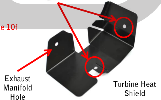
M6x1.0x10mm Cap Screws
